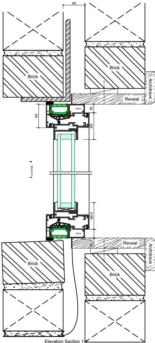
Elevation Section 1-1
