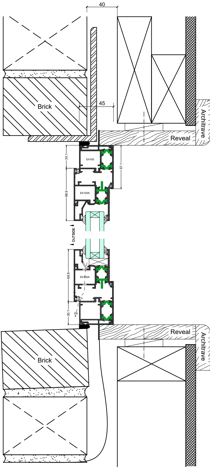
Elevation Section 1-1
