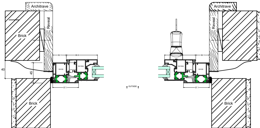
Plan Section 2-2
