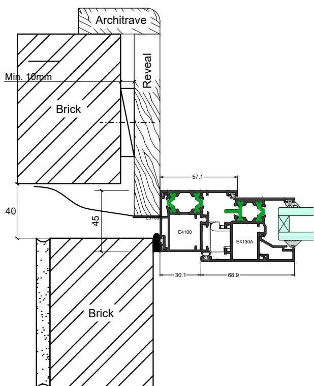
Elevation Section 1-1
