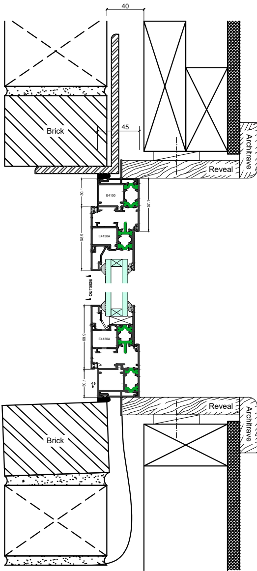
Elevation Section 1-1
