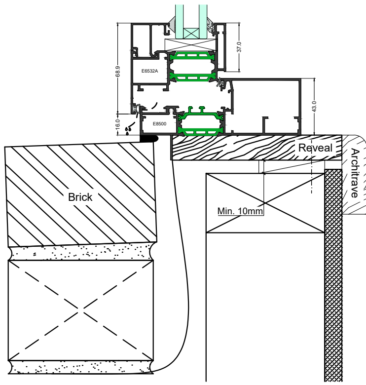
Elevation Section 1-1
