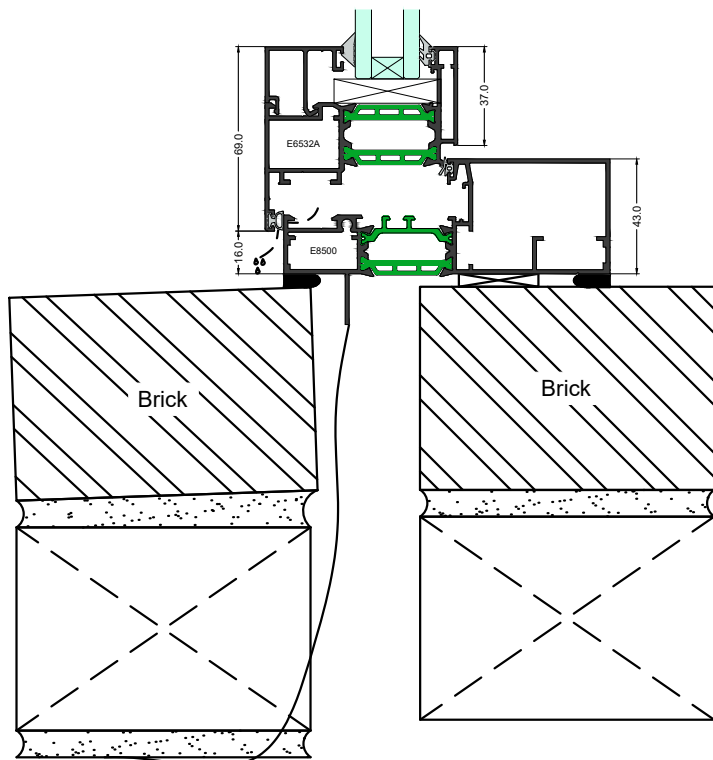
Elevation Section 1-1
