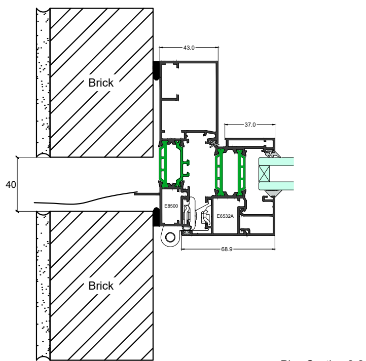
Plan Section 2-2
