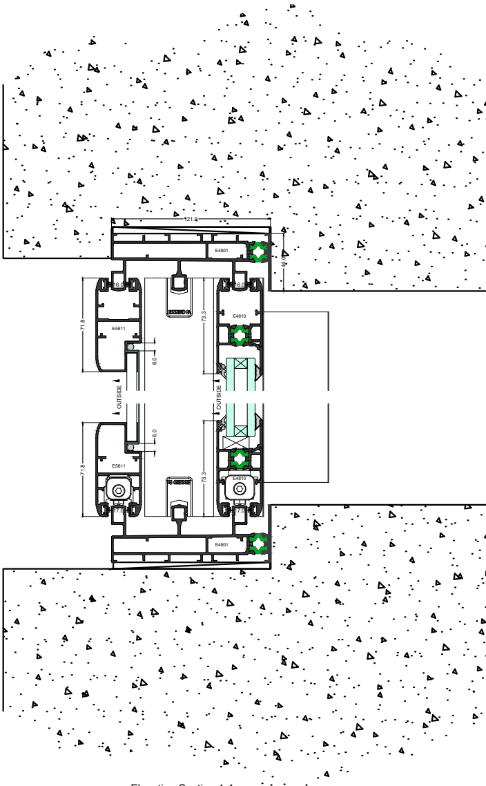
Elevation Section 1-1
