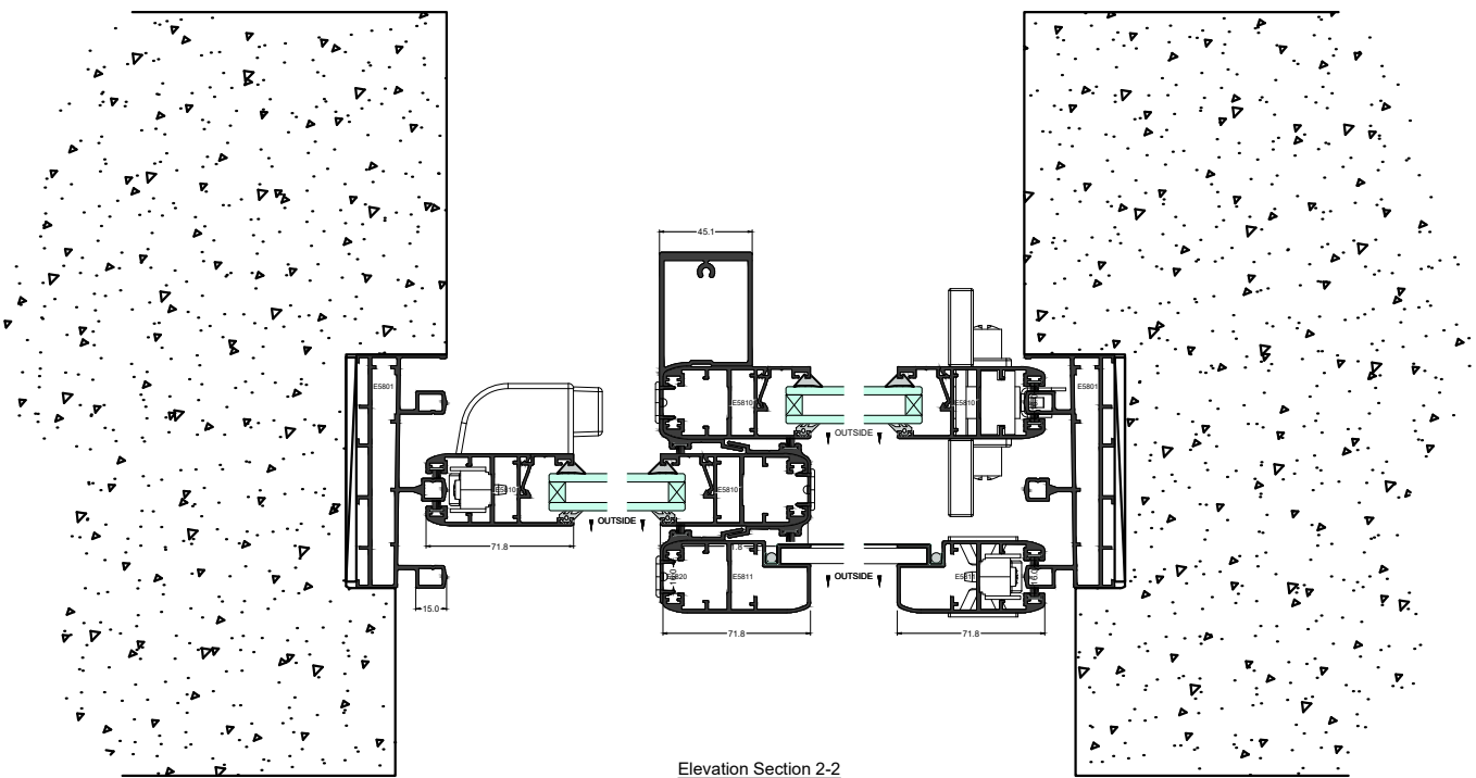
Elevation Section 2-2
