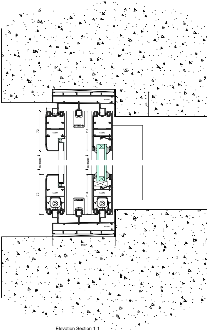
Elevation Section 1-1
