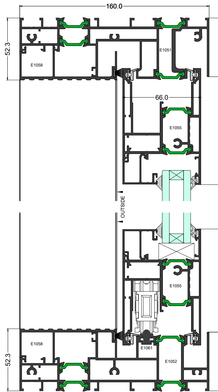
Elevation Section 1-1
