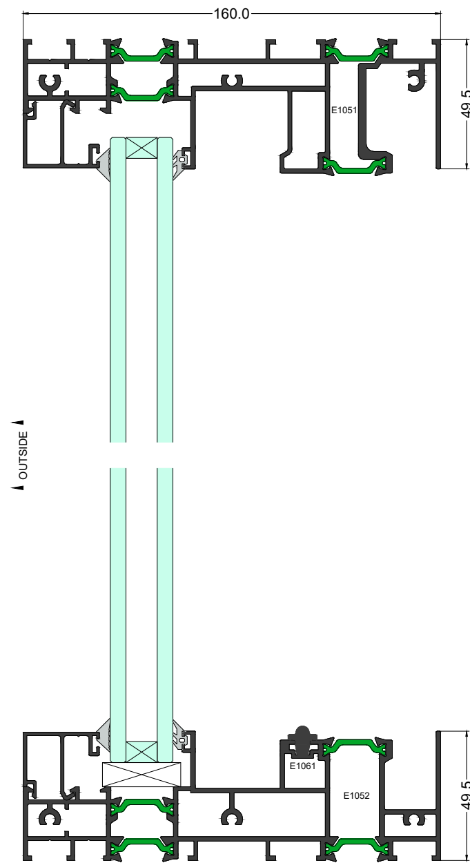
Elevation Section 2-2
