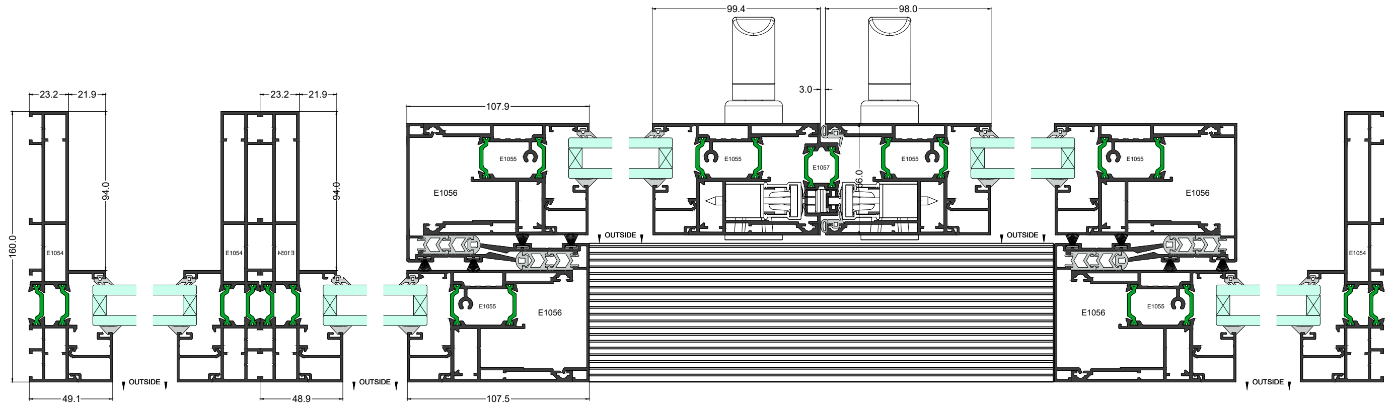
Plan Section 9-9
