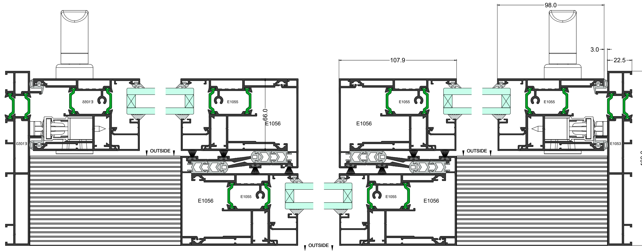
Plan Section 5-5
