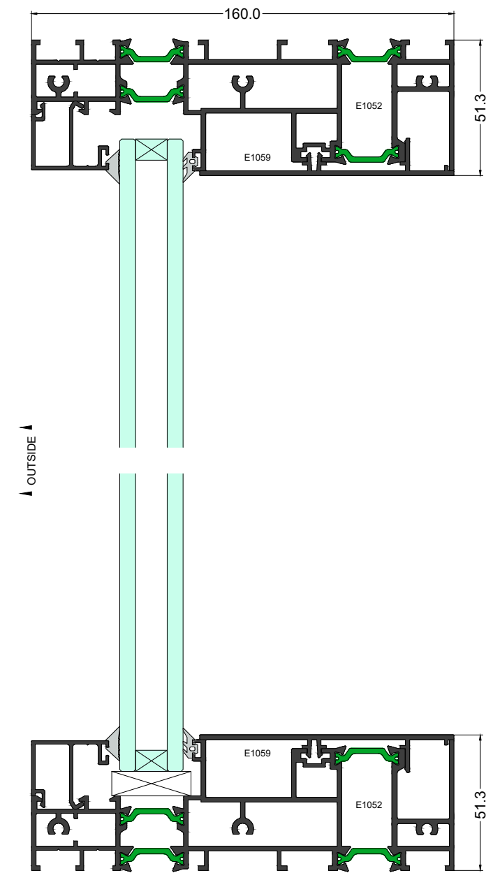
Elevation Section 8-8
