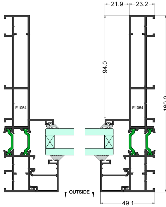
Plan Section 7-7
