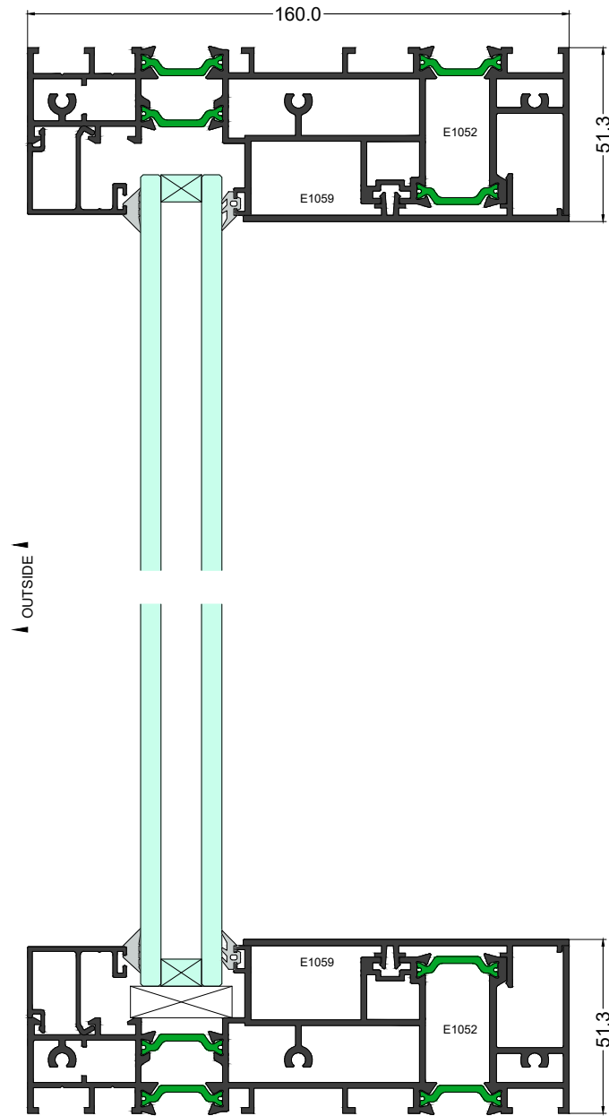
Elevation Section 8-8
