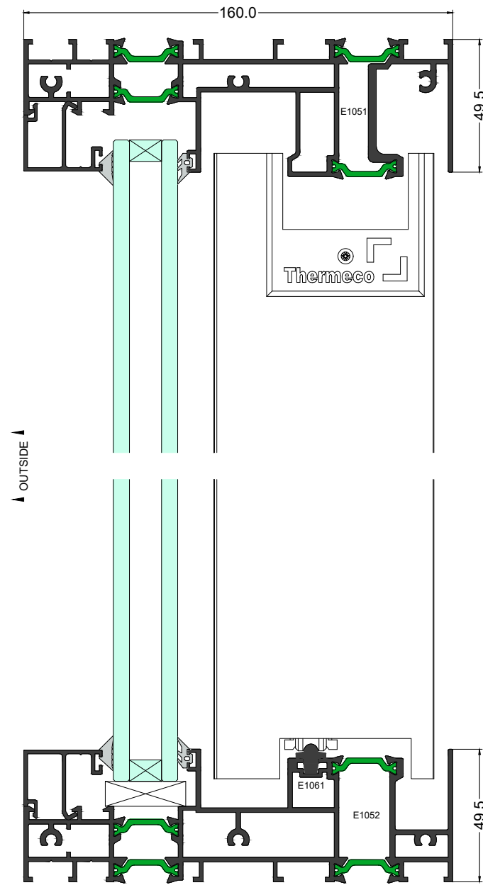
Elevation Section 4-4
