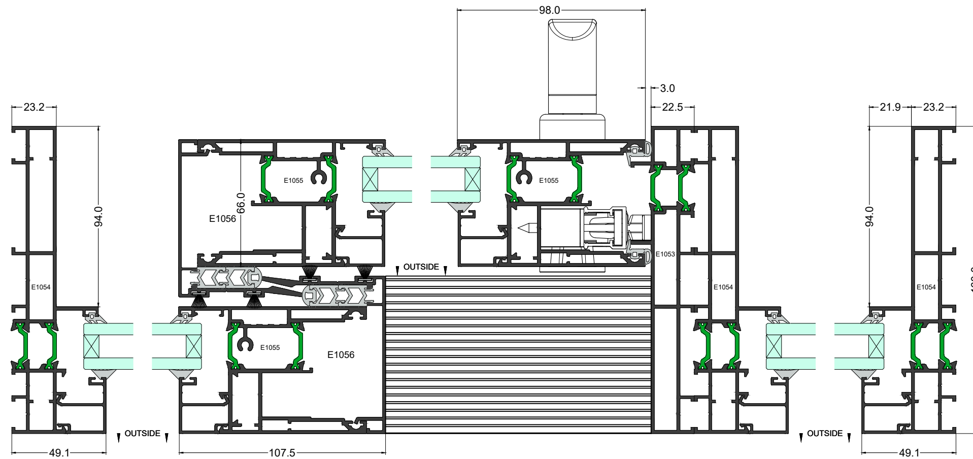
Plan Section 10-10
