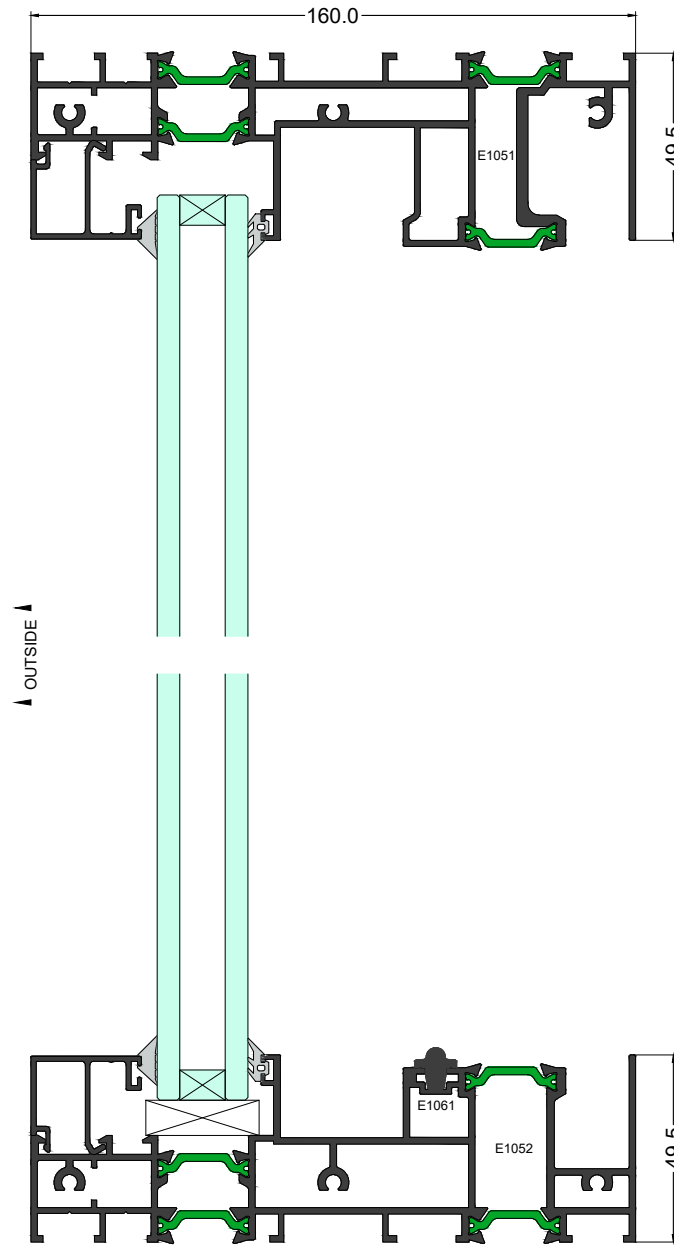
Elevation Section 2-2
