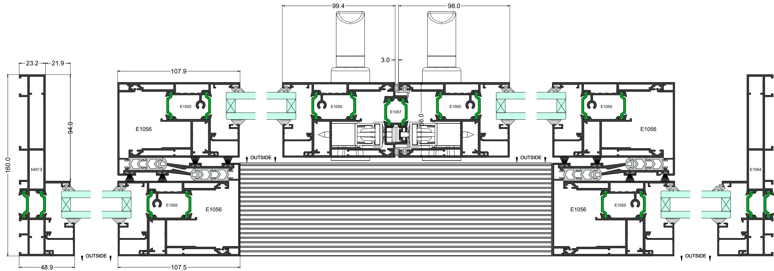
Plan Section 6-6
