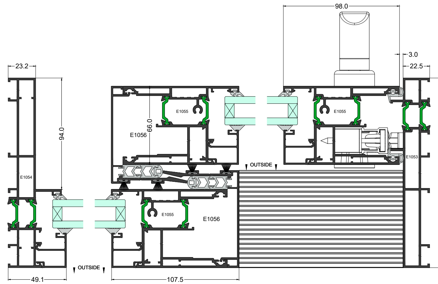
Plan Section 3-3
