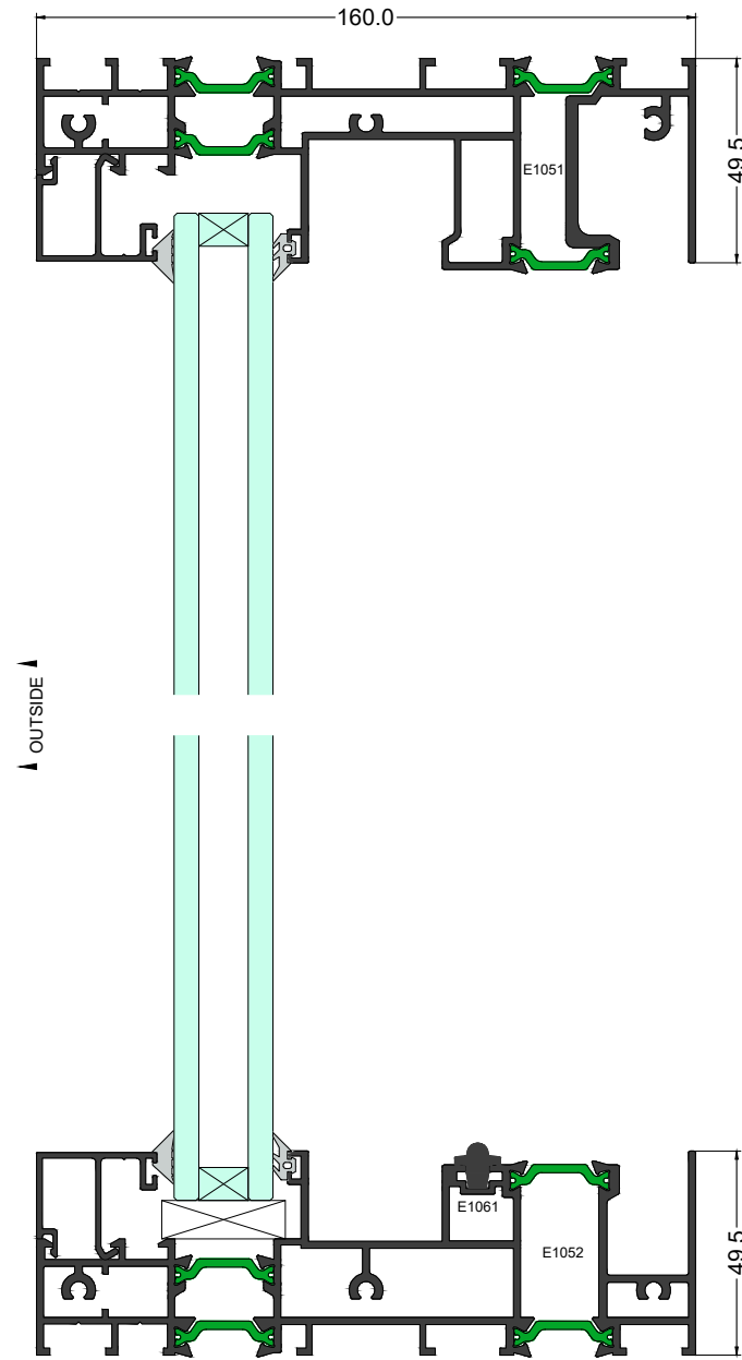
Elevation Section 2-2
