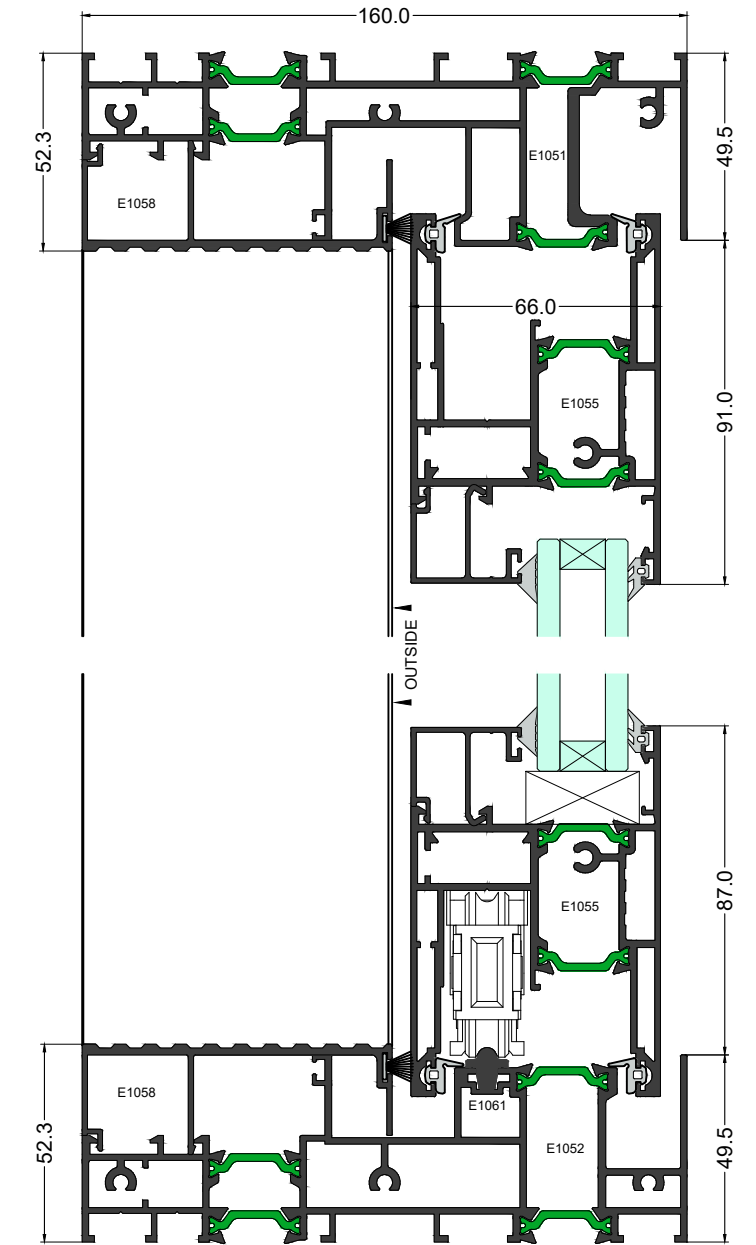
Elevation Section 1-1
