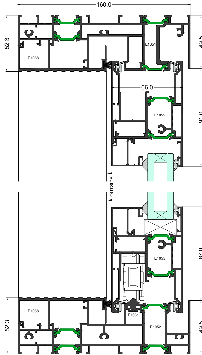
Elevation Section 1-1
