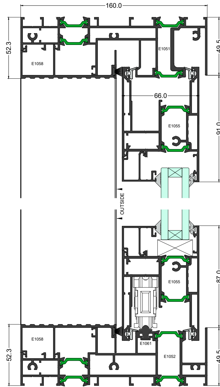
Elevation Section 1-1
