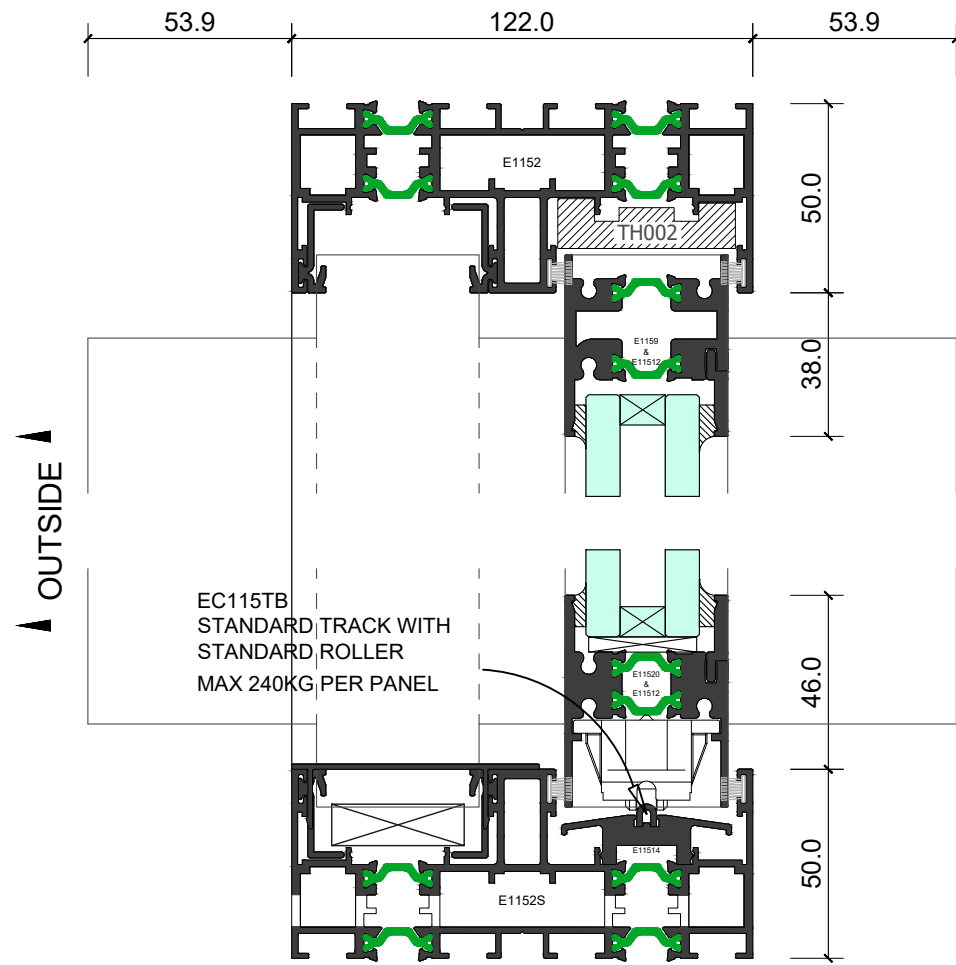
Elevation Section 2-2
