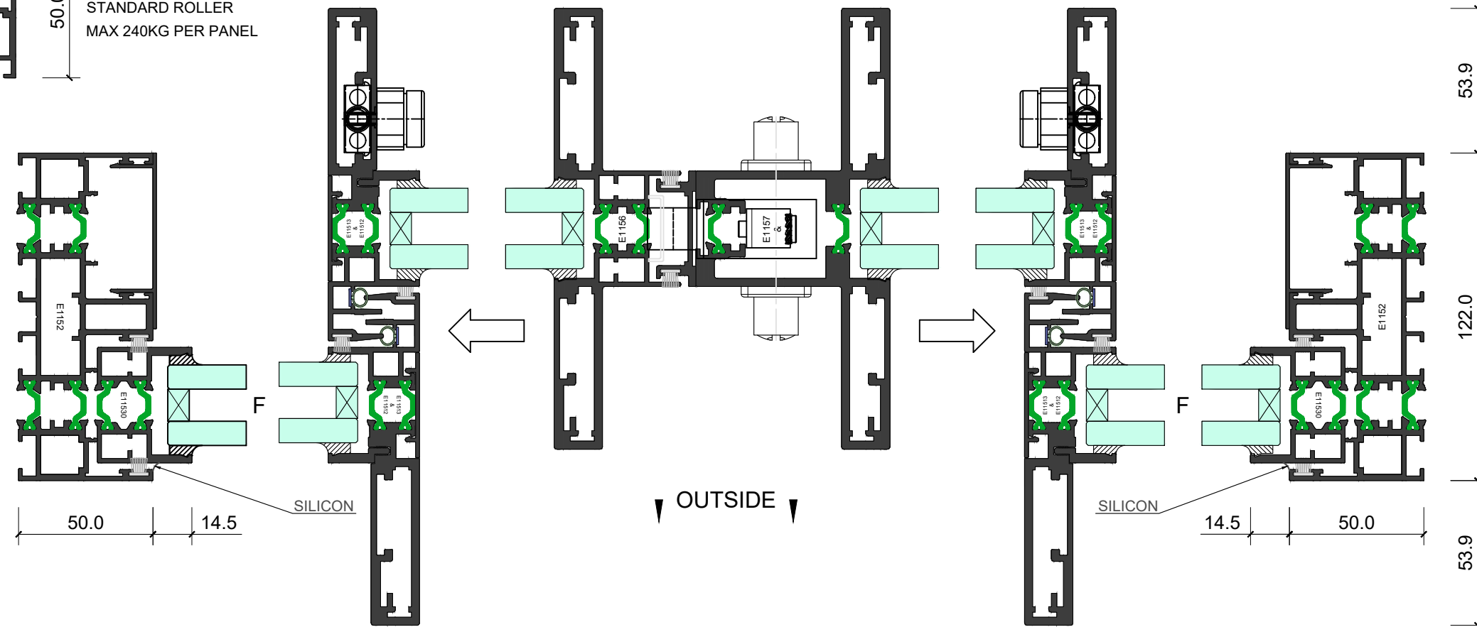
Plan Section 1-1
