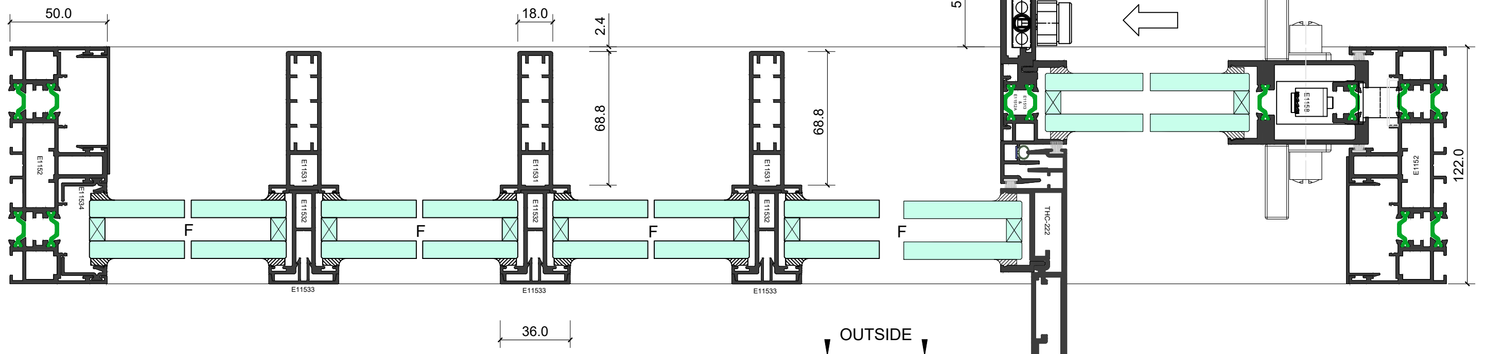
Plan Section 1-1
