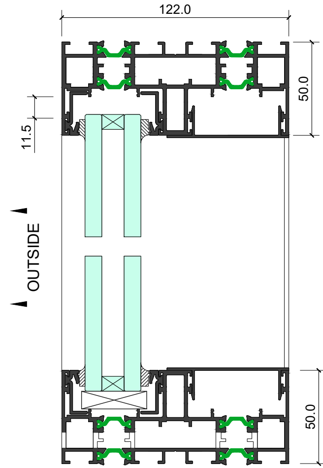
Elevation Section 2-2
