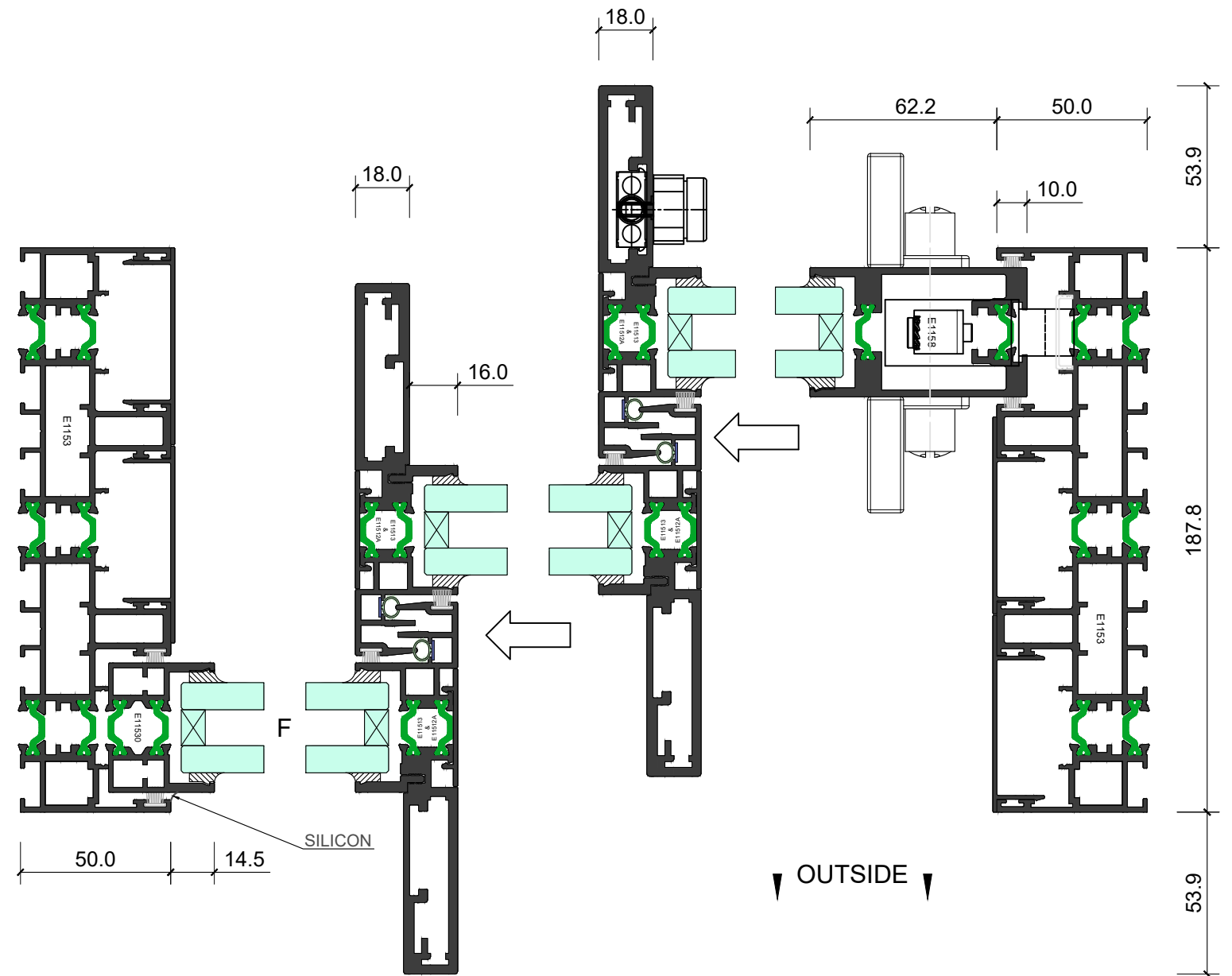
Plan Section 1-1
