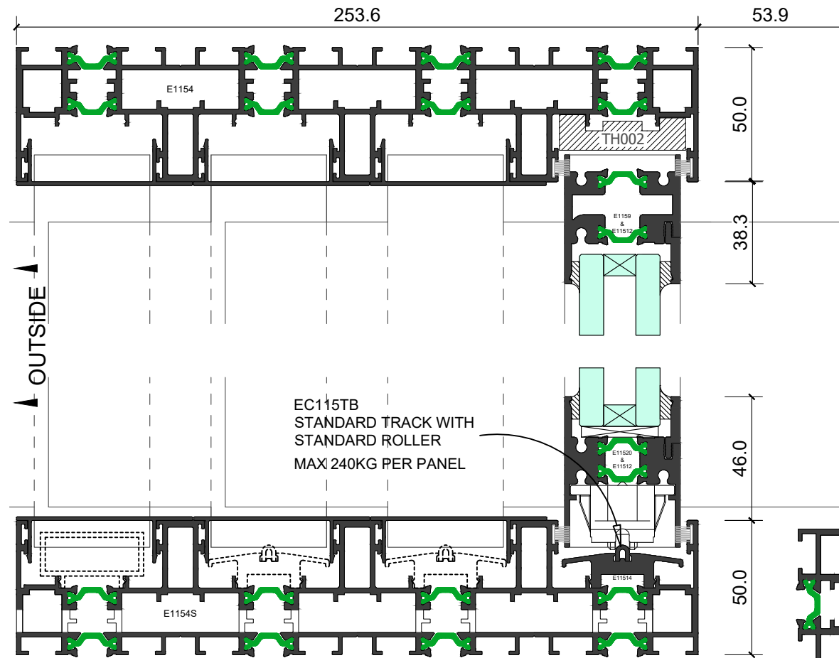
Elevation Section 2-2
