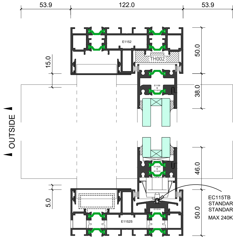
Elevation Section 2-2
