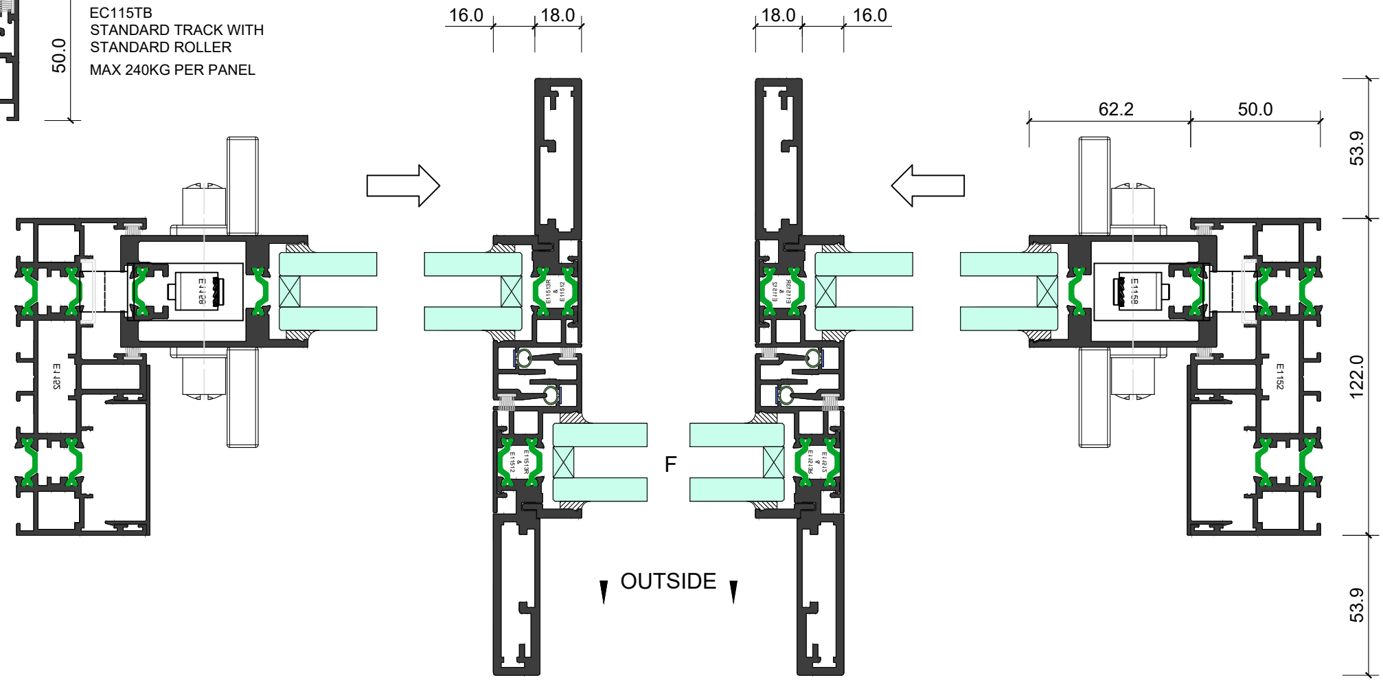
Plan Section 1-1
