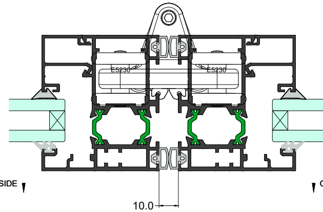
Plan Section 4-4
