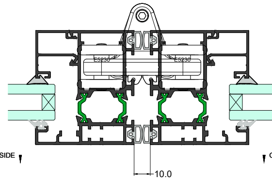
Plan Section 5-5
