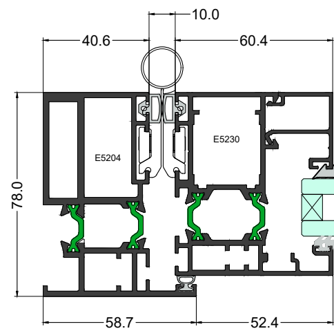
Elevation Section 1-1
