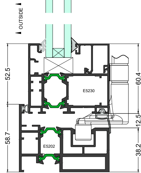
Elevation Section 1-1
