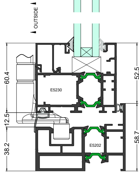
Elevation Section 1-1
