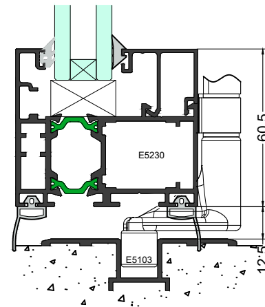
Alternative Sill
