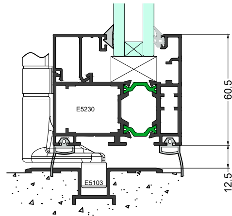
Alternative Sill
