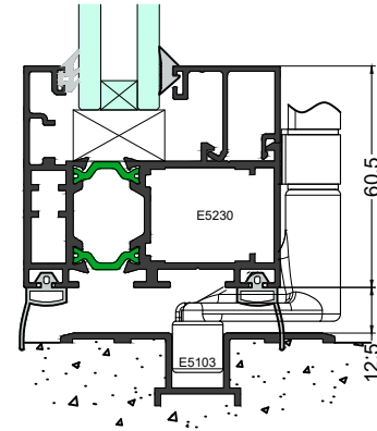
Alternative Sill
