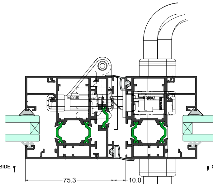
Plan Section 6-6
