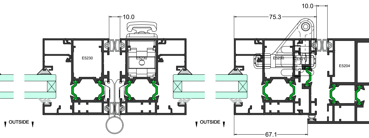
Plan Section 2-2
