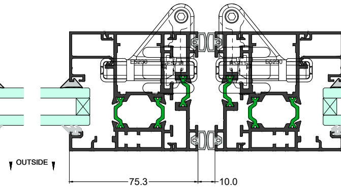
Plan Section 3-3
