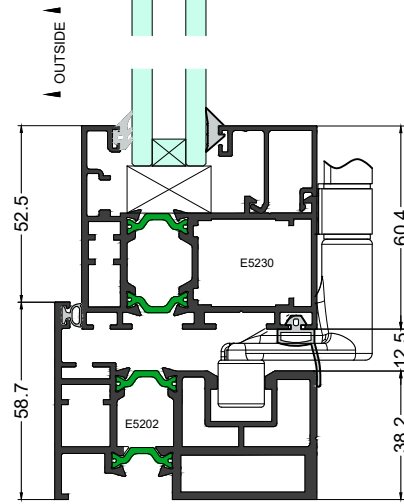
Elevation Section 1-1
