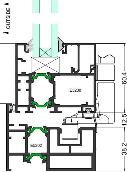
Elevation Section 1-1
