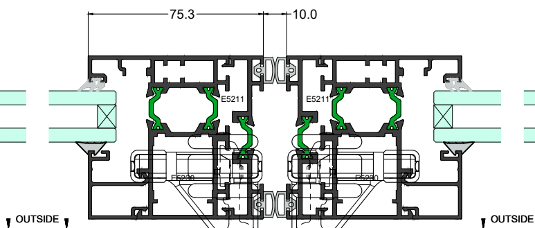
Plan Section 3-3
