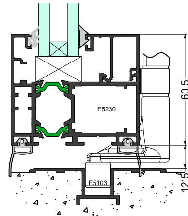
Alternative Sill
