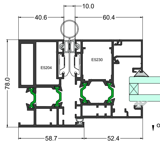
Elevation Section 1-1
