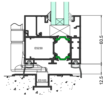
Alternative Sill
