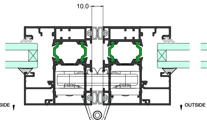
Plan Section 4-4
