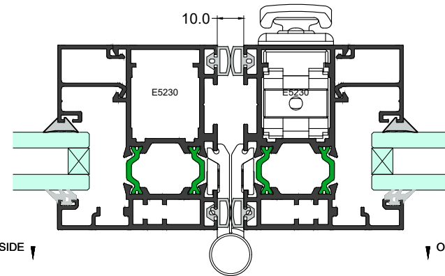
Plan Section 6-6
