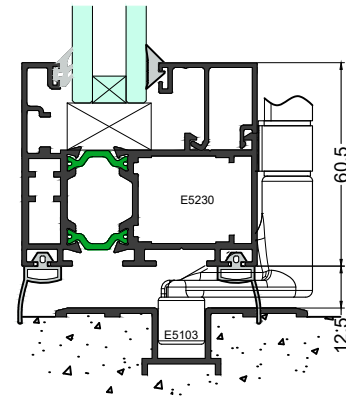
Alternative Sill
