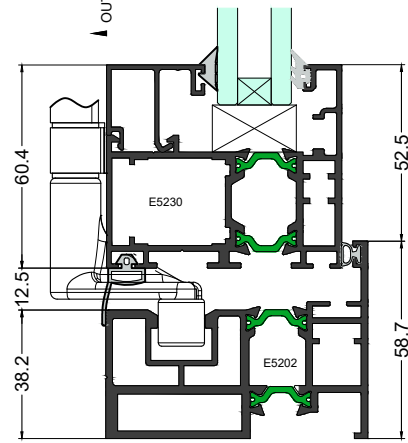
Elevation Section 1-1
