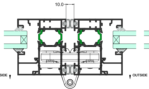
Plan Section 5-5
