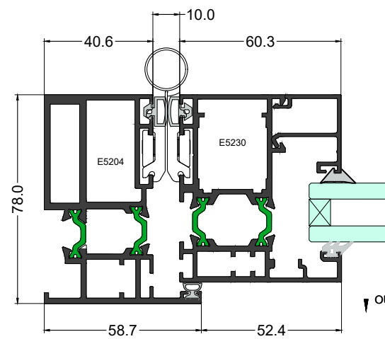
Elevation Section 1-1
