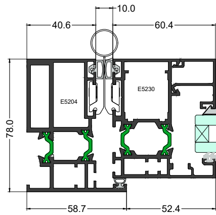
Elevation Section 1-1
