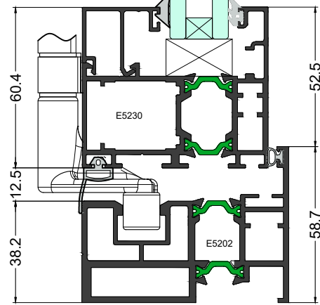
Elevation Section 1-1
