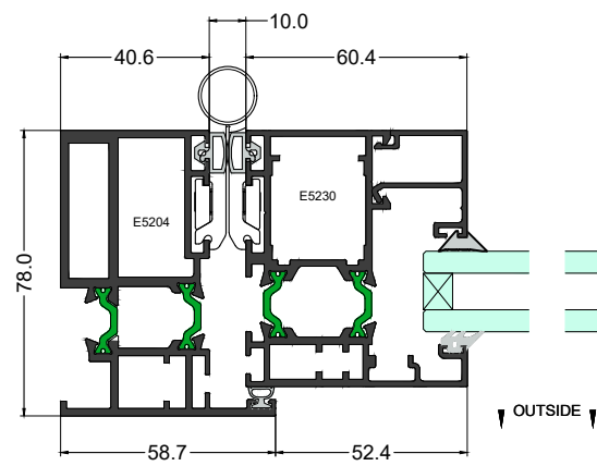
Elevation Section 1-1
