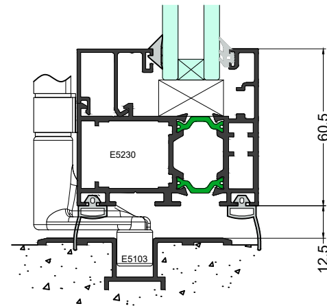
Alternative Sill
