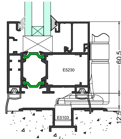
Alternative Sill
